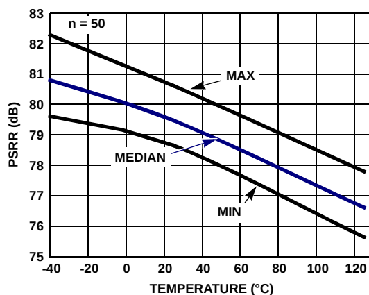
FIGURE 26. PSRR vs TEMPERATURE \pm 1.5V TO \pm 2.5V
