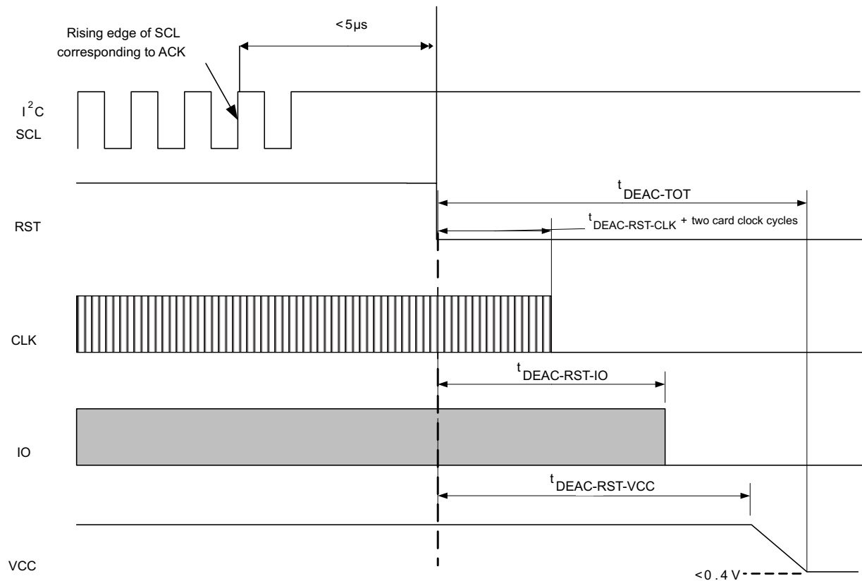
Figure 8. Card Deactivation Sequence Initiated by I²C Command
