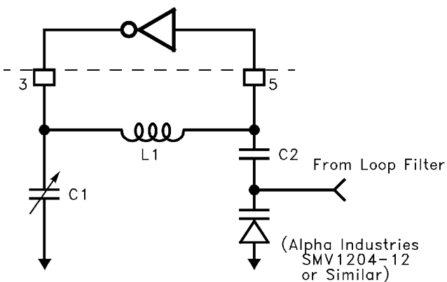
FIGURE 12. TYPICAL LC VCO
