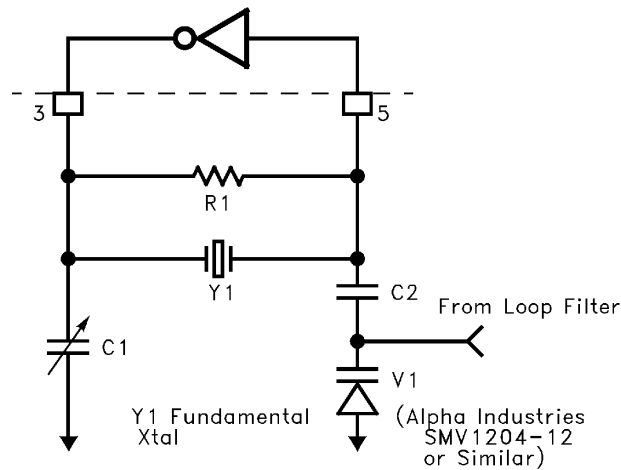
FIGURE 13. TYPICAL XTAL VCO
