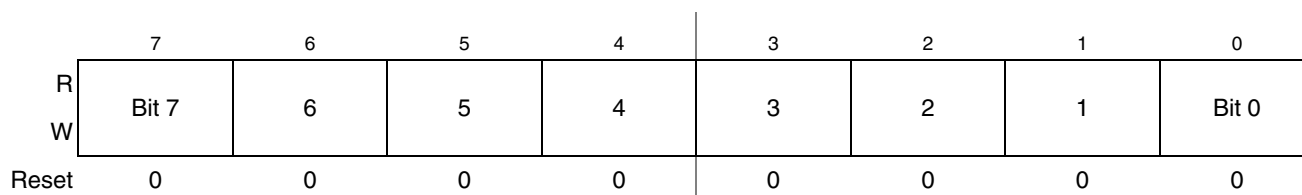
Figure 15-14. TPM Channel Value Register Low (TPMxCnVL)
