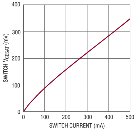
Switch V_{\text{CESAT}}
