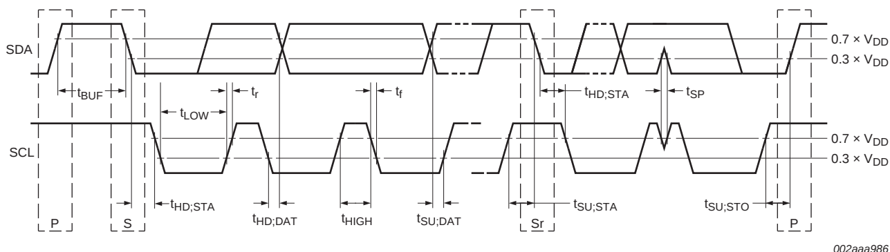
Fig 18. Definition of timing
