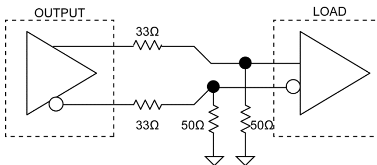
PCI-Express Device Routing
