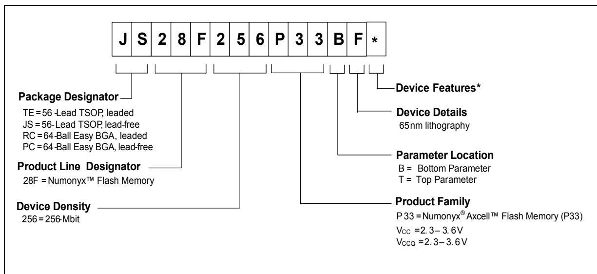
Figure 28: Decoder for Discrete Products
