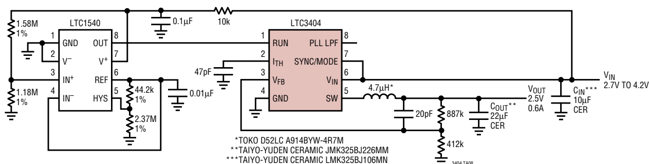
Single Li-Ion to 2.5V/0.5A Regulator with Precision 2.7V Undervoltage Lockout
