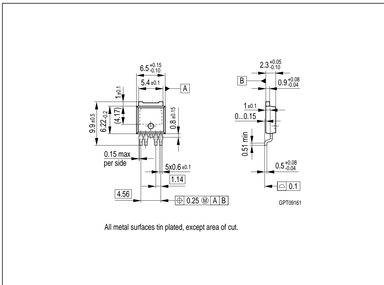
Figure 4 P-T0252-5-1 (Plastic Transistor Single Outline)
