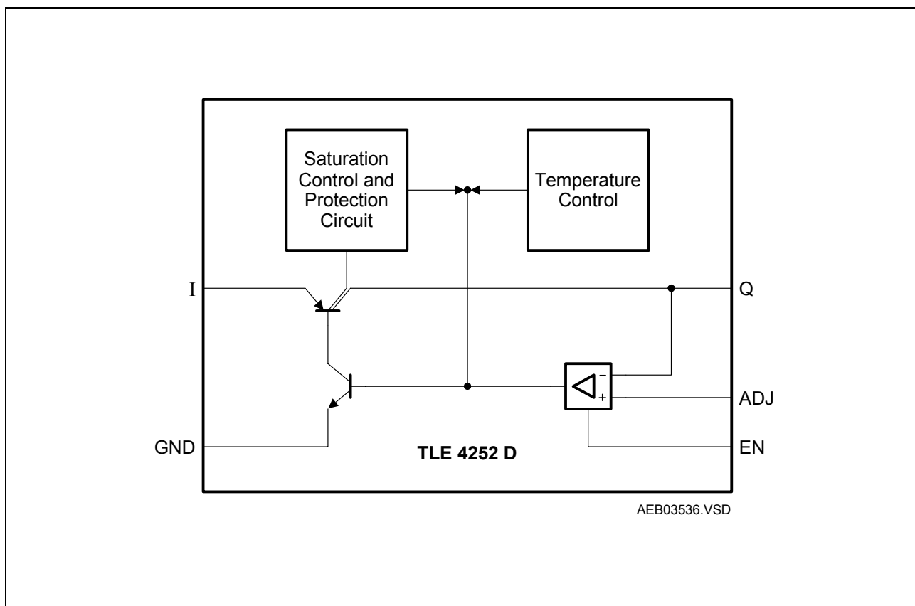
Figure 1 Internal Circuit Blocks
