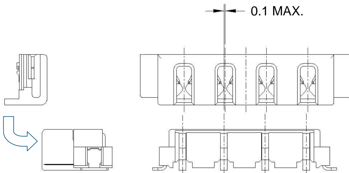
Fig.3-1 Displacement allowance for durability test
