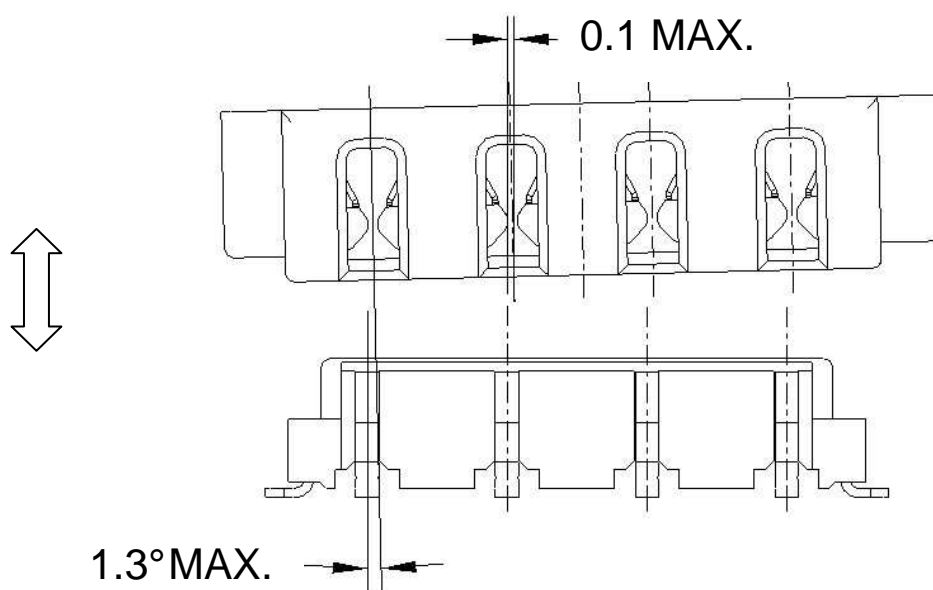
Fig.3-2 Tilt allowance for durability test
