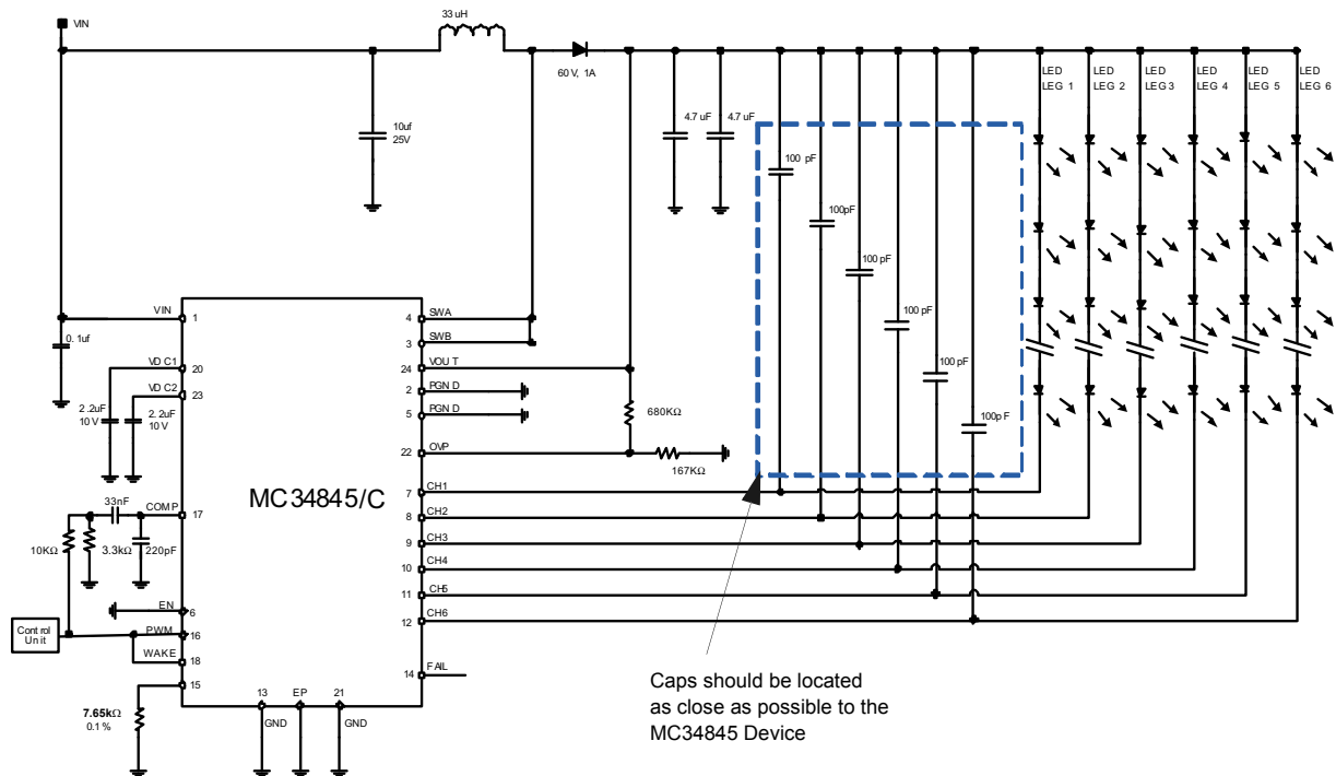
Figure 10. Typical Application Circuit for Single Wire Control, f_s = 600 \text{ KHz} ( V_{IN} = 9.0\text{V} , I_{LED}/\text{channel} = 20 \text{ mA}/\text{channel} , 10 LEDs/channel, OVP = 35V, V_{PWM} = 3.3\text{V} )
