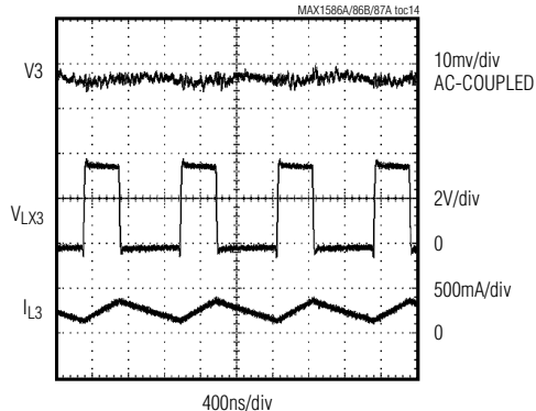
REG3 SWITCHING WAVEFORMS WITH 250mA LOAD
