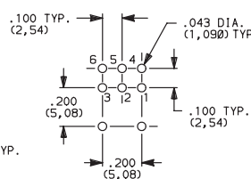
T201MH9ABE Horizontal Actuation DPDT
