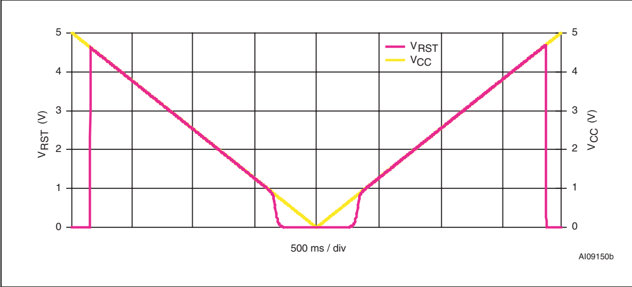
Figure 21. \text{RST} output voltage vs. supply voltage
