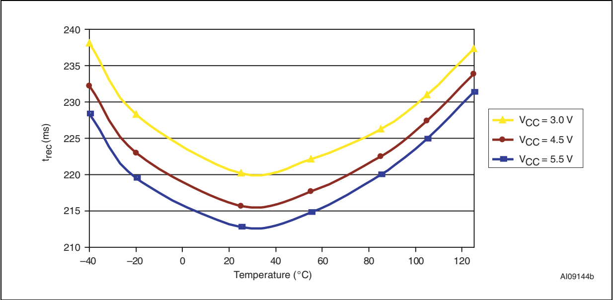
Figure 15. Power-up t_{\text{rec}} vs. temperature
