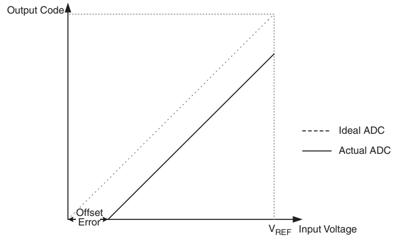
Figure 22-10. Offset Error
