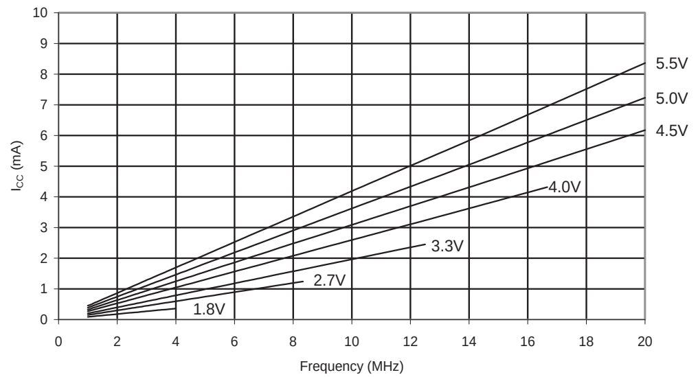
Figure 29-7. Idle Supply Current vs. Frequency (1 MHz - 20 MHz)
