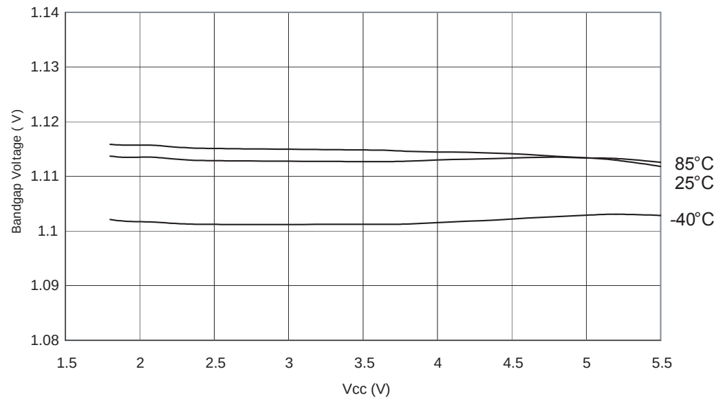
Figure 29-50. Bandgap Voltage vs. V_{CC}
