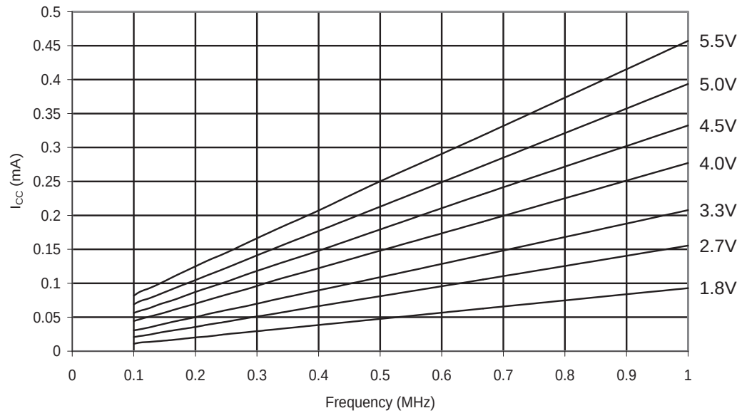
Figure 29-6. Idle Supply Current vs. Frequency (0.1 MHz - 1.0 MHz)
