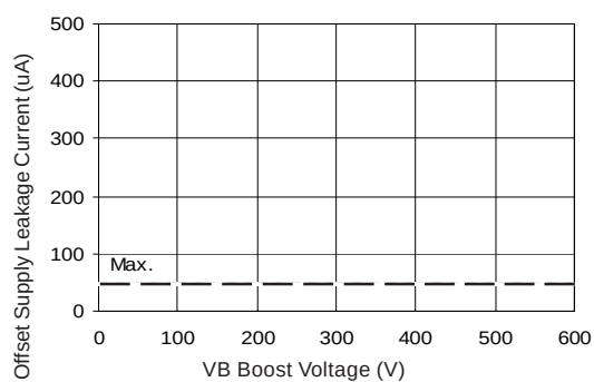
Figure 22B Offset Supply Current vs Voltage
