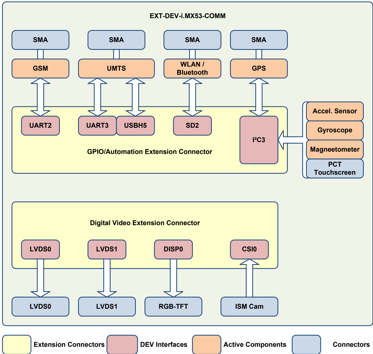
Figure 2-1: Interconnection Diagram
