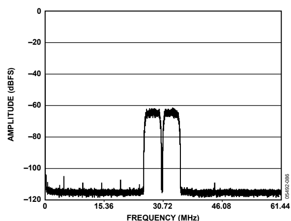
Figure 26. AD9233-125 Two 64k WCDMA Carriers with F_{IN} = 215.04 MHz, F_S = 122.88 MSPS
