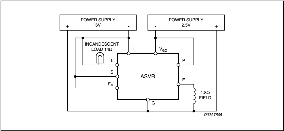
Figure 4. Reverse B+ Test Circuit
