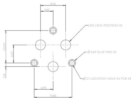
PCB HOLE & GLUE PAD LOCATION
