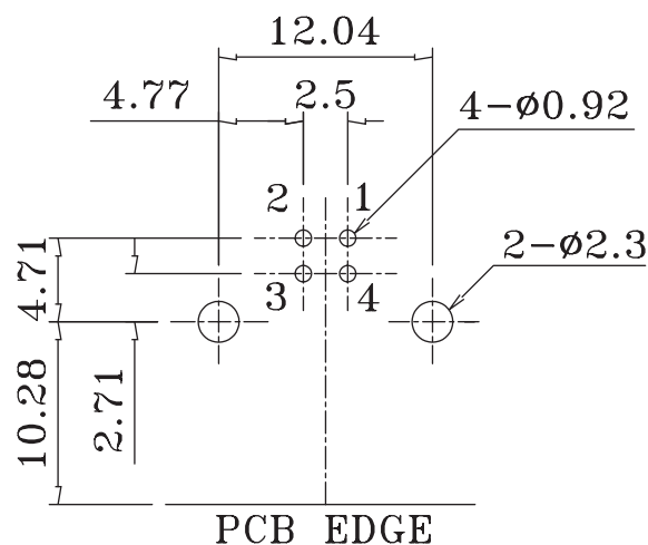
PC Board Layout - Component Side
