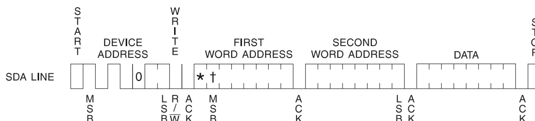
Figure 8. Byte Write
