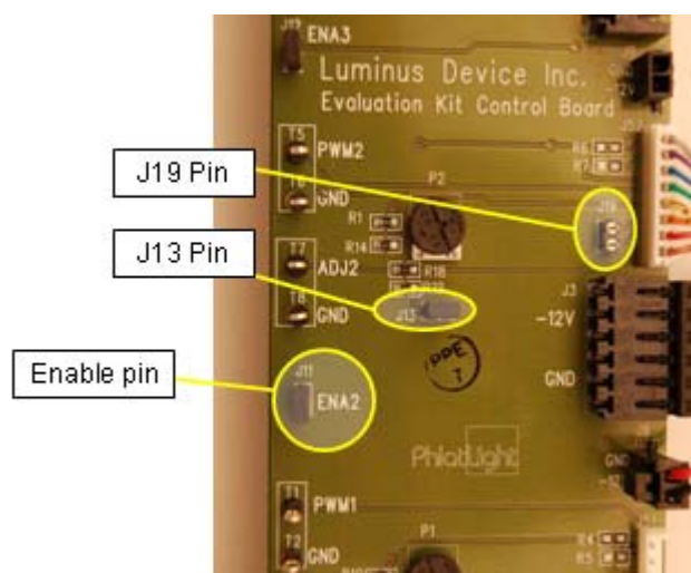
Figure 16: Jumper Locations
