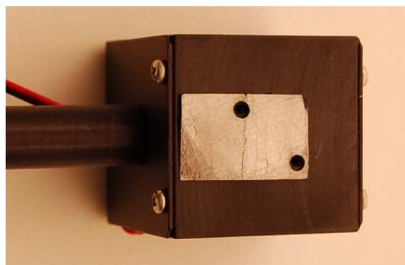
Figure 8: C21 package type thermal interface material placed on heat sink
