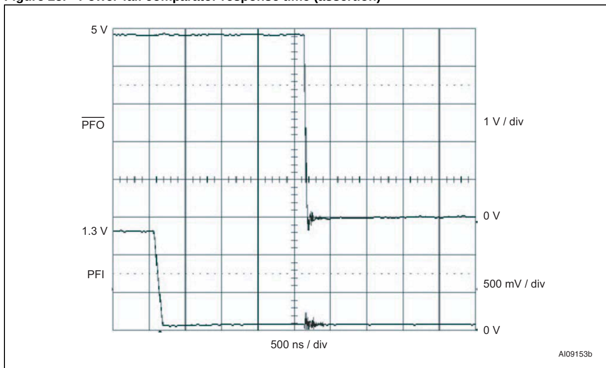
Figure 25. Power-fail comparator response time (assertion)
