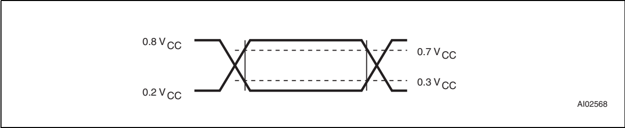
Figure 28. AC testing input/output waveforms
