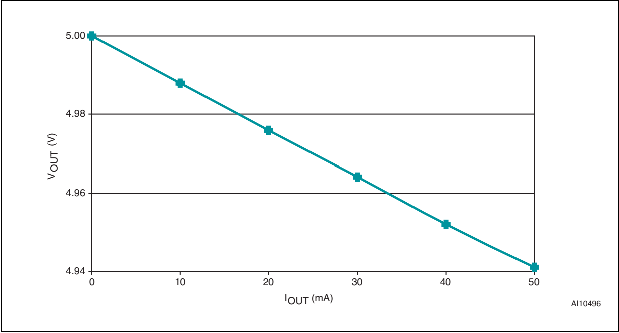
Figure 19. Output voltage vs. load current ( V_{\text{CC}} = 5\text{ V} ; V_{\text{BAT}} = 2.8\text{ V} ; T_{\text{A}} = 25\text{ °C} )
