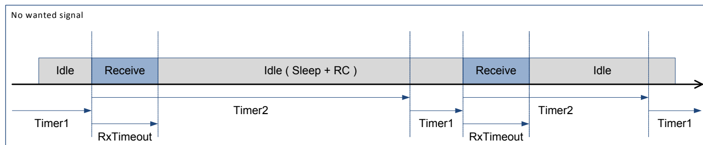
Figure 51. Listen Mode with no SyncAddress Detected
