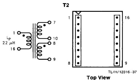
FIGURE 22. Pulse PE-68412 (Surface Mount)
