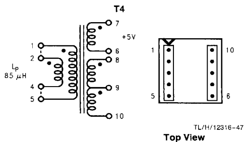
FIGURE 32. Schott 67140930
