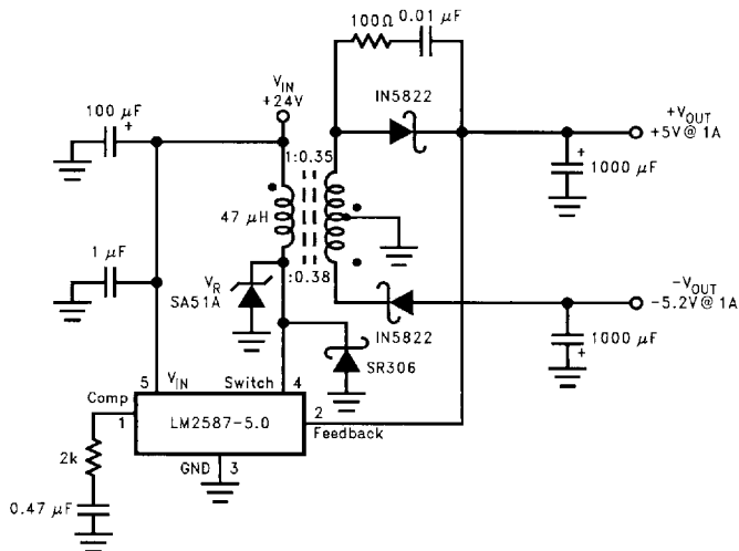
FIGURE 42. Flyback Regulator
