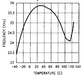
Short Circuit Frequency vs Temperature
