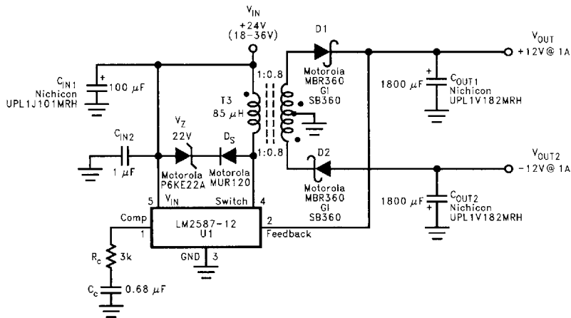
FIGURE 11. Dual-Output Flyback Regulator
