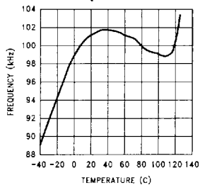
Oscillator Frequency vs Temperature
