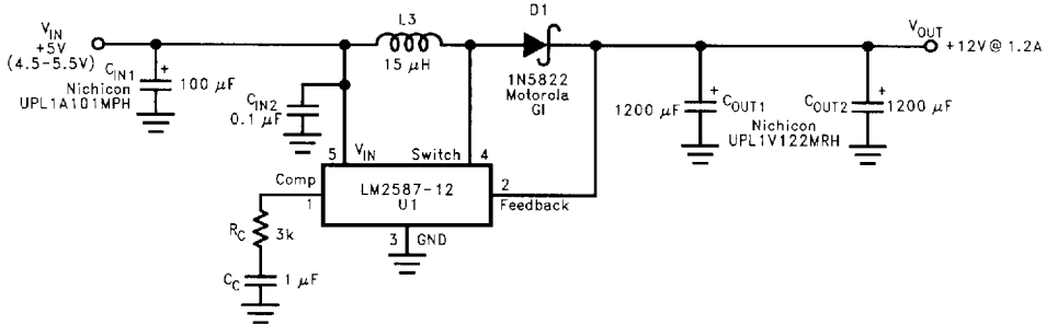
FIGURE 36. +5V to +12V Boost Regulator
