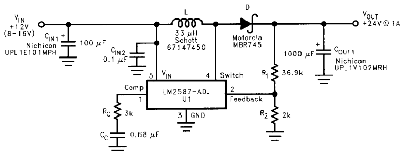
FIGURE 38. +12V to +24V Boost Regulator
