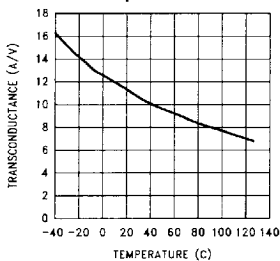
Switch Transconductance vs Temperature
