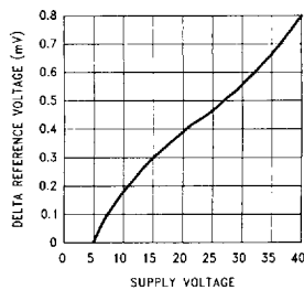
ΔReference Voltage vs Supply Voltage
