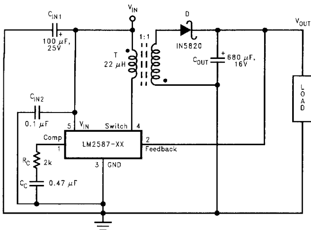
FIGURE 2. LM2587-3.3 and LM2587-5.0
