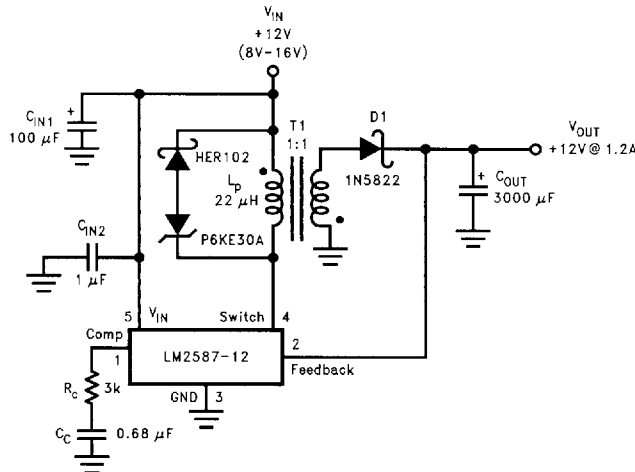
FIGURE 4. 12V Flyback Regulator Design Example
