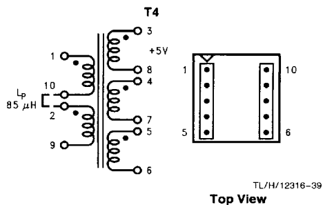
FIGURE 24. Pulse PE-68422 (Surface Mount)
