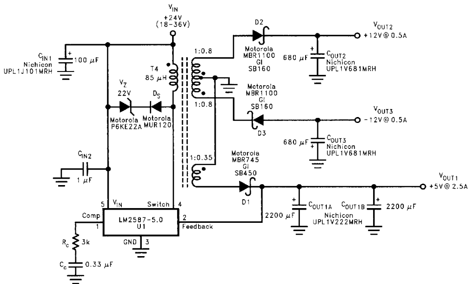
FIGURE 12. Triple-Output Flyback Regulator
