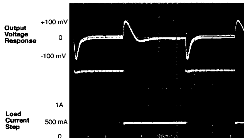
FIGURE 35. V_{OUT} Response to Load Current Step
