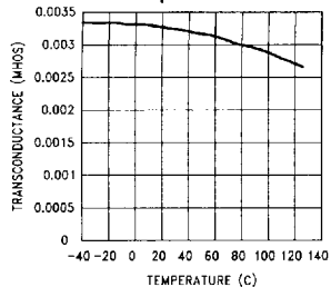
Error Amp Transconductance vs Temperature
