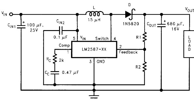
FIGURE 3. LM2587-12 and LM2587-ADJ
