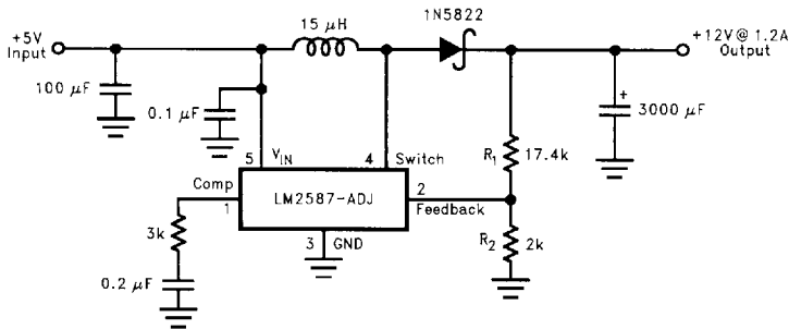
FIGURE 41. Boost Regulator
