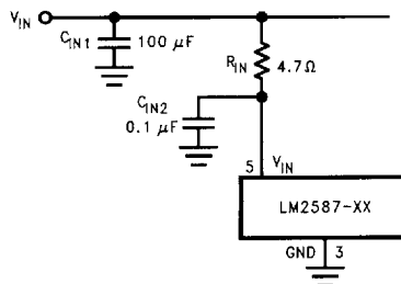
FIGURE 43. Input Line Filter
