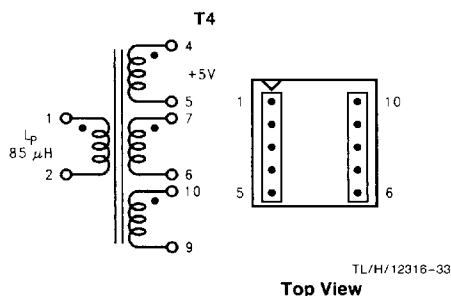
FIGURE 18. Coilcraft Q4344-B
