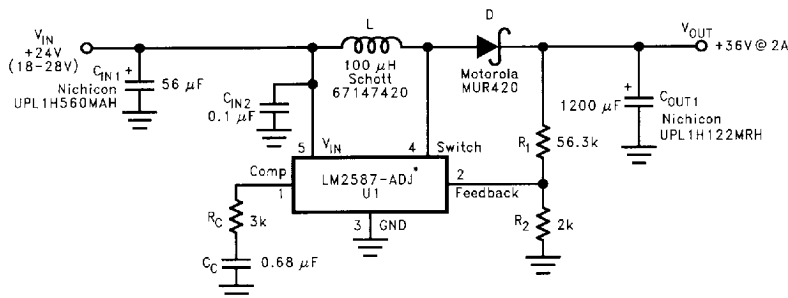
FIGURE 39. +24V to +36V Boost Regulator
