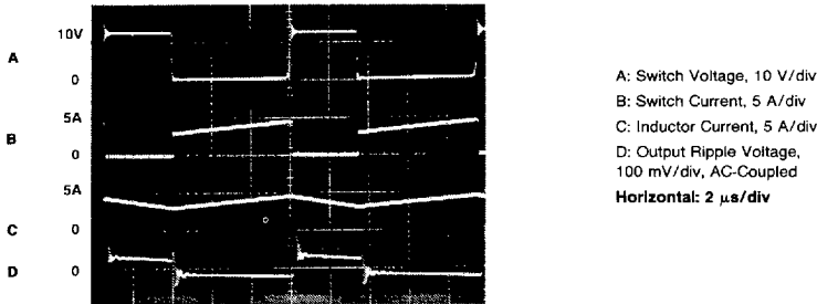
FIGURE 34. Switching Waveforms
