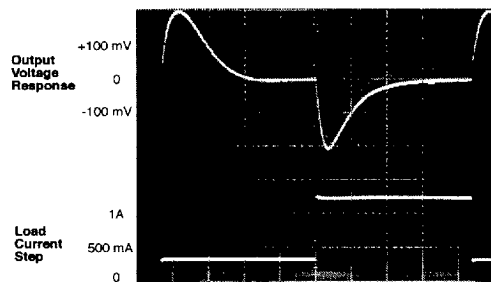
FIGURE 6. V_{OUT} Load Current Step Response
