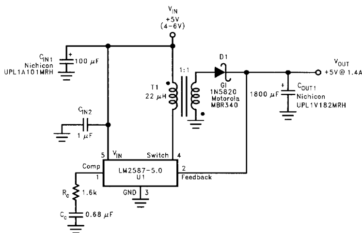
FIGURE 8. Single-Output Flyback Regulator
