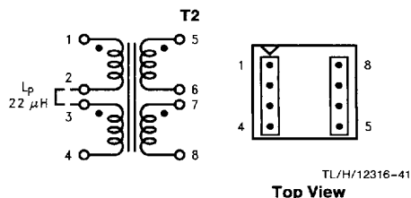
FIGURE 26. Renco RL-5531
