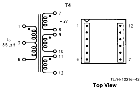
FIGURE 28. Renco RL-5535
