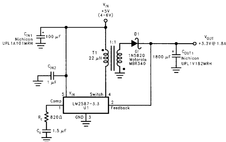
FIGURE 7. Single-Output Flyback Regulator
