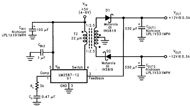
FIGURE 10. Dual-Output Flyback Regulator
