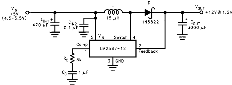
FIGURE 33. 12V Boost Regulator
