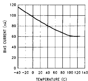
Feedback Pin Bias Current vs Temperature
