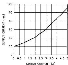
Supply Current vs Switch Current
