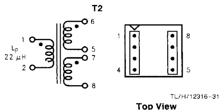
FIGURE 16. Coilcraft Q4337-B
