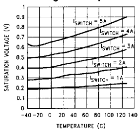
Switch Saturation Voltage vs Temperature
