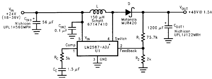
FIGURE 40. +24V to +48V Boost Regulator
