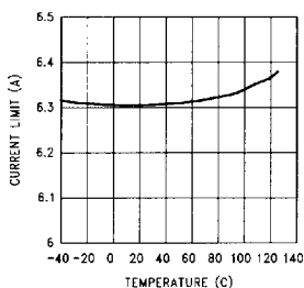
Current Limit vs Temperature
