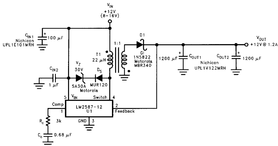
FIGURE 9. Single-Output Flyback Regulator
