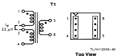
FIGURE 25. Renco RL-5530
