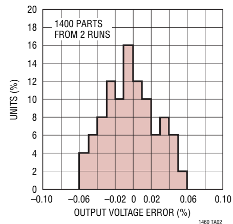
Typical Distribution of Output Voltage S8 Package
