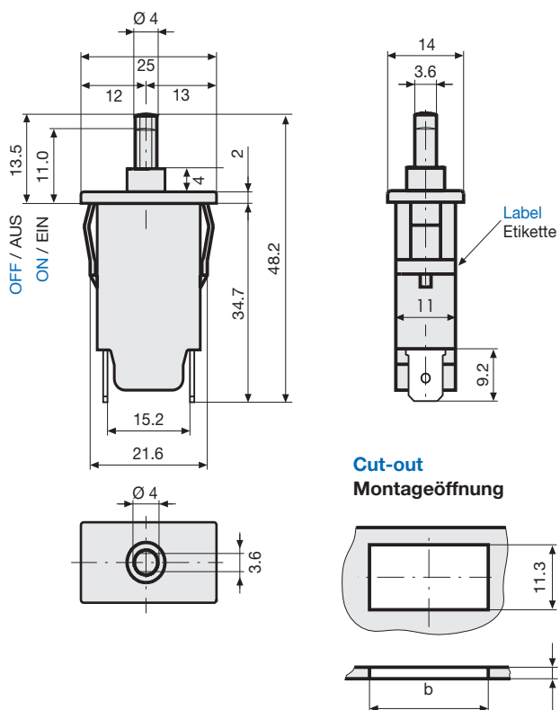
T11-611 ≤7,5 A
