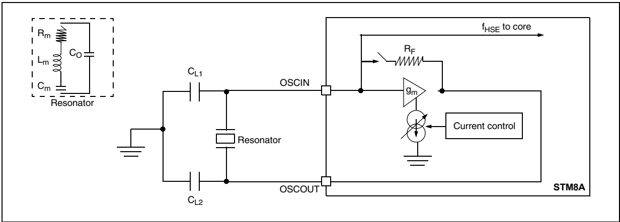
Figure 16. HSE oscillator circuit diagram
