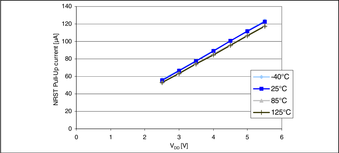
Figure 34. Typical NRST pull-up current I_{pu} vs V_{DD}
