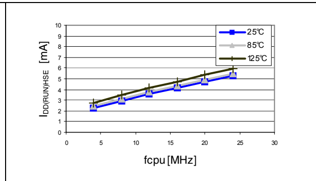
Figure 10. Typ. I_{DD(RUN)HSE} vs. f_{CPU} @ V_{DD} = 5.0 V, periph = on
