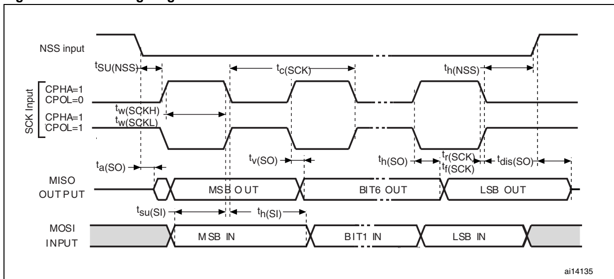
Figure 37. SPI timing diagram where slave mode and CPHA = 1
