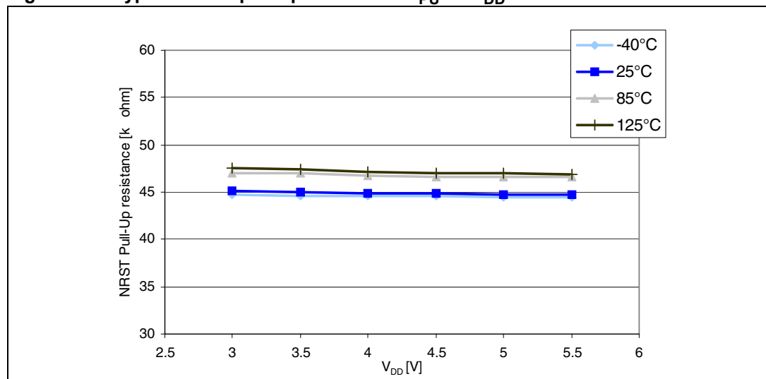
Figure 33. Typical NRST pull-up resistance R_{PU} vs V_{DD}
