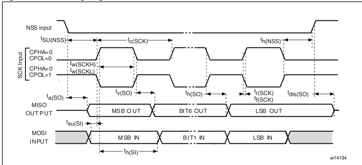
Figure 36. SPI timing diagram where slave mode and CPHA = 0
