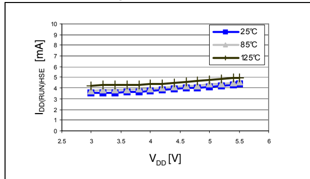
Figure 9. Typ. I_{DD(RUN)HSE} vs. V_{DD} @ f_{CPU} = 16 MHz, periph = on
