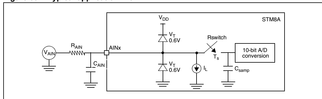
Figure 39. Typical application with ADC
