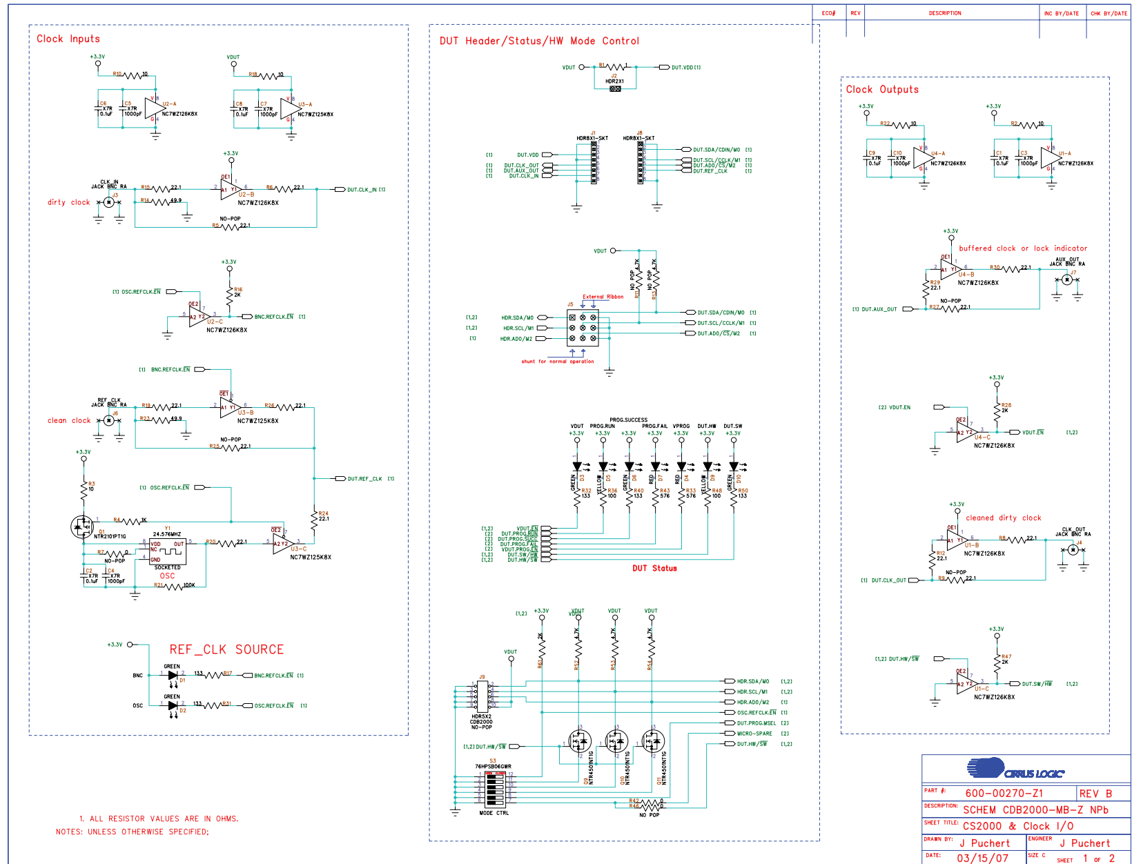
Figure 5. CDB2000-MB Schematic Page 1
