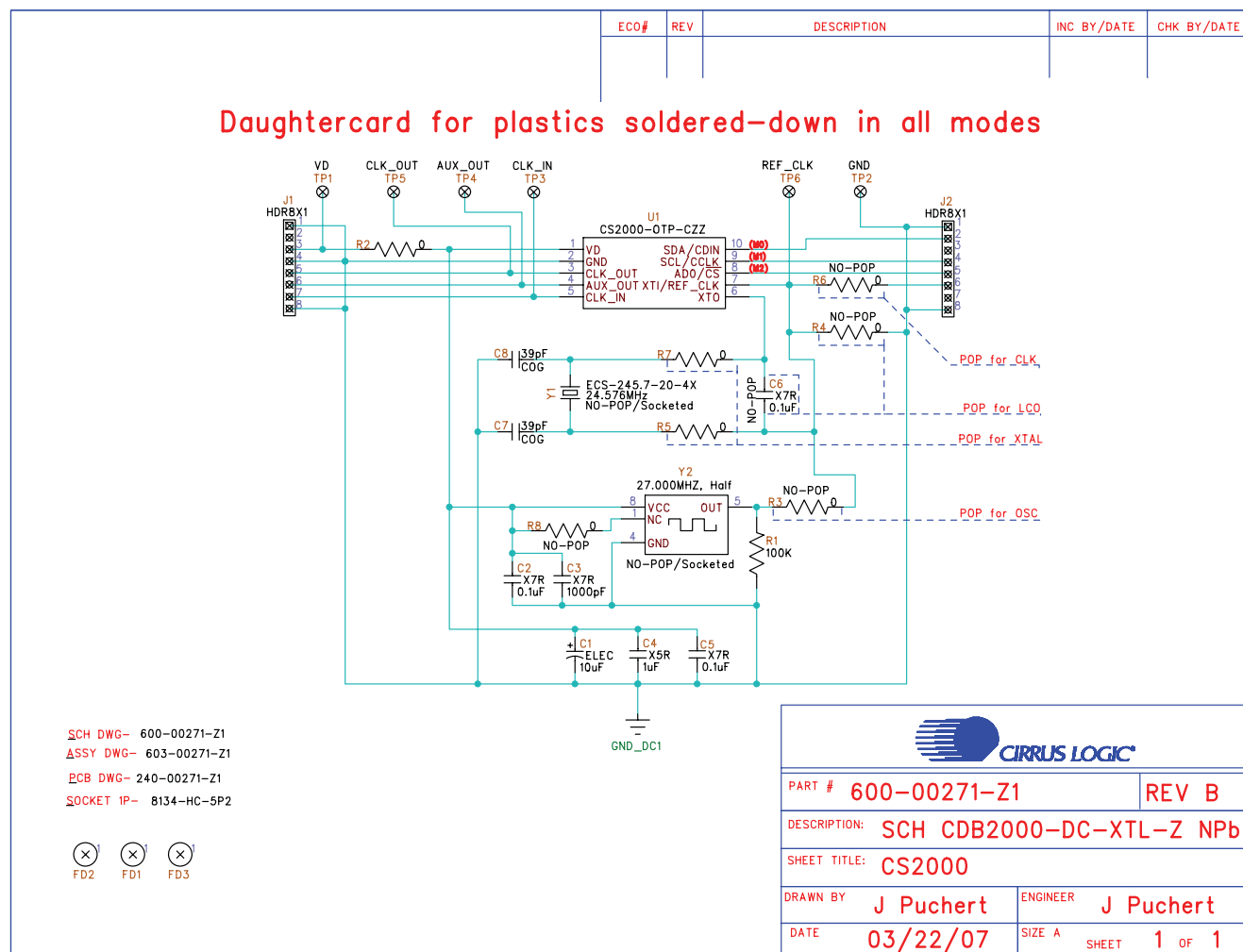
Figure 12. CDB2000-DC Schematics
