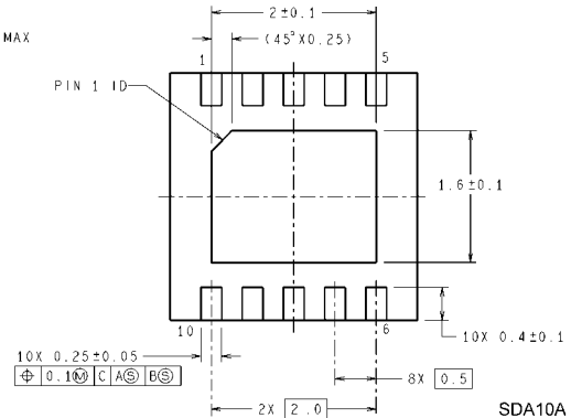
LLP, 10 Lead, Package NS Package Number SDA10A
