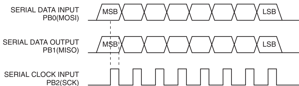
Figure 30. Low-voltage Serial Programming Waveforms
