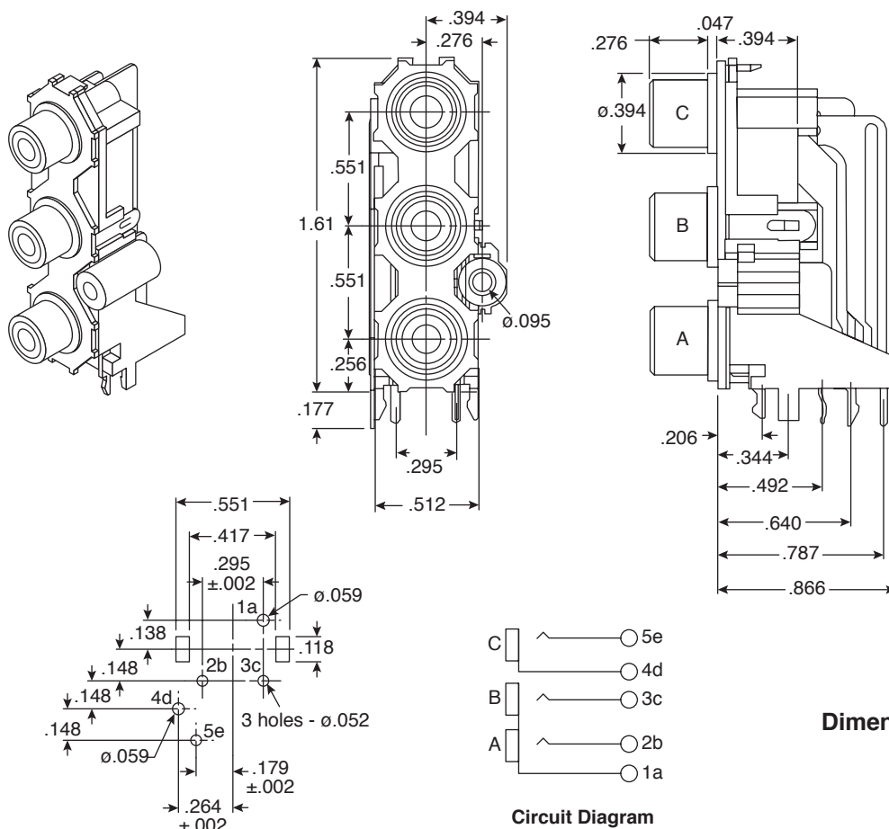
PCB Hole Layout (Bottom View)
