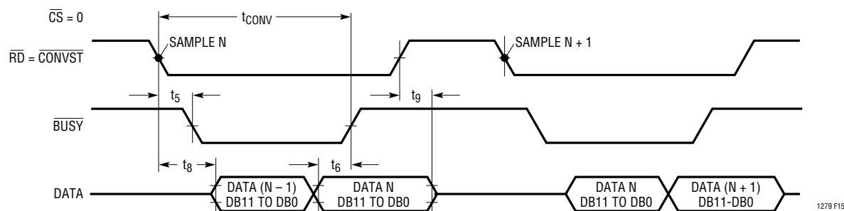
Figure 15. Slow Memory Mode
