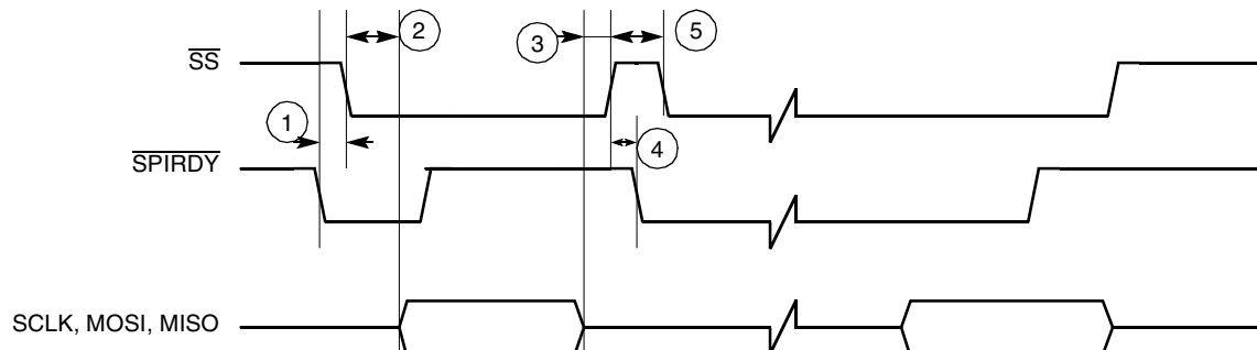
Figure 14. Master CSPI Timing Diagram Using \overline{\text{SPI\_RDY}} Edge Trigger
