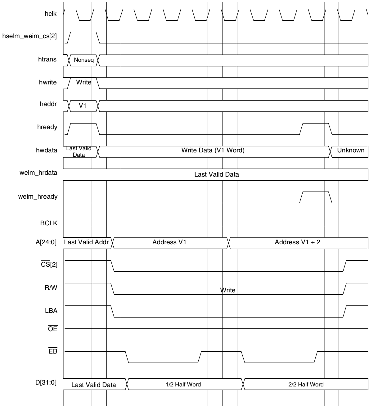
Figure 64. WSC = 2, WWS = 1, WEA = 1, WEN = 2, A.WORD/E.HALF
