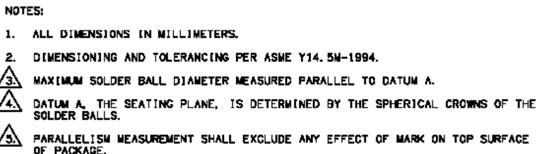
Figure 86. i.MX21 MAPBGA Mechanical Drawing
