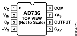
Figure 2. Pin Configuration
