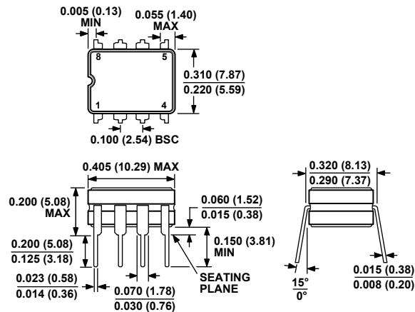
Figure 27. 8-Lead Ceramic Dual In-Line Package [CERDIP]
