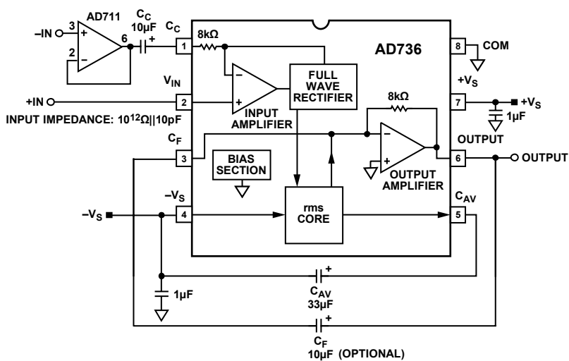
Figure 22. Differential Input Connection
