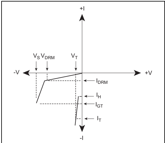
V-I Characteristics for Negative Battrax
