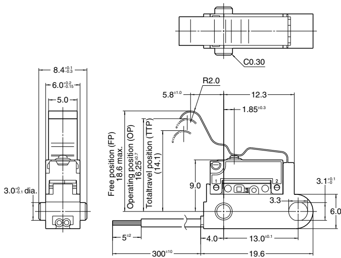
External dimensions
