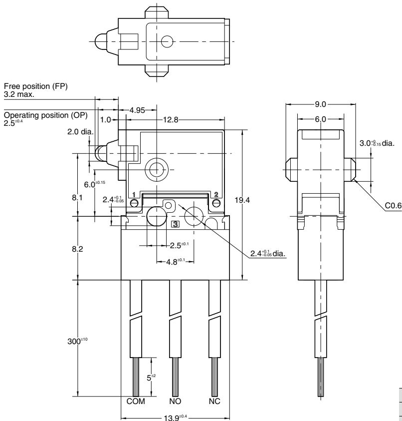
External dimensions
