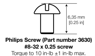
Figure 14. Screw Dimensions
