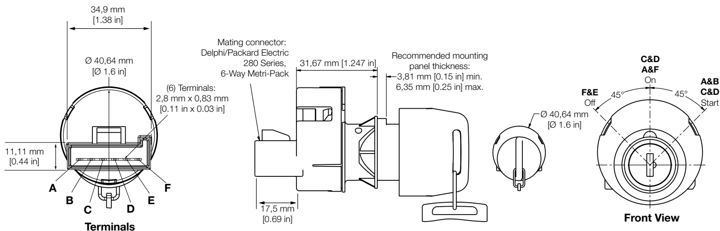
Figure 3. Model 89165 Key Switch Dimensions
