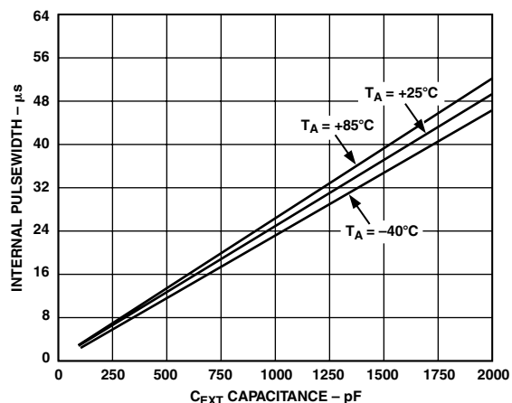
Figure 7. Internal Pulsewidth vs. \text{C}_{\text{EXT}}
