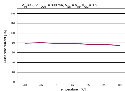
Figure 16. Quiescent current vs. temperature ( I_{OUT} = 300\text{ mA} , normal mode)
