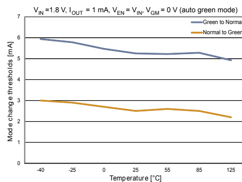
Figure 14. Mode change thresholds vs. temperature
