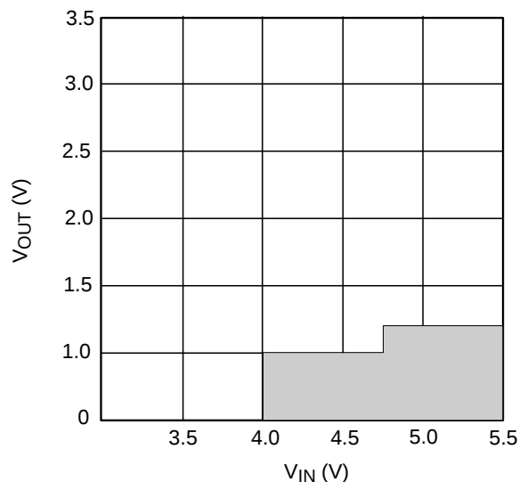
Figure 40. LP3906 Buck Converter V_{OUT} vs V_{IN} Operating Range during PFM-PWM-PPM Transition
