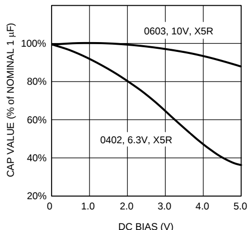
Figure 39. Graph Showing a Typical Variation in Capacitance vs. DC Bias
