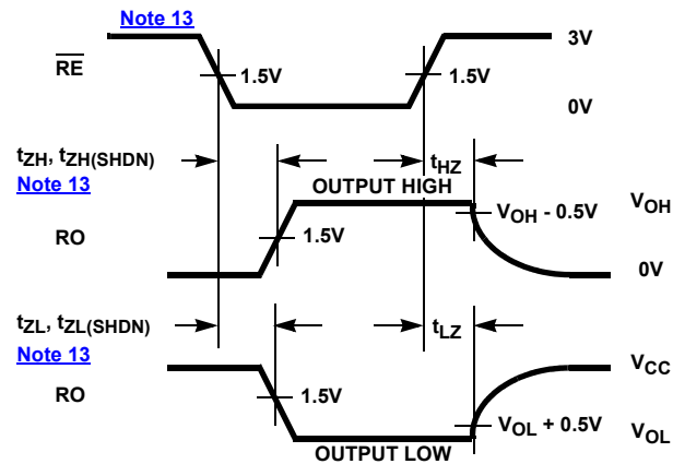
FIGURE 10. RECEIVER ENABLE AND DISABLE TIMES
