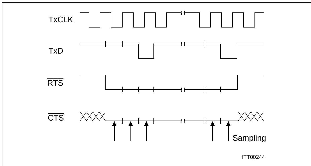
Figure 59 \overline{RTS}/\overline{CTS} Handshaking
