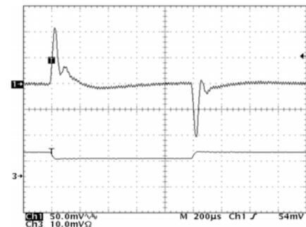
Figure 14. EMS10DG, Load Response (typ)
