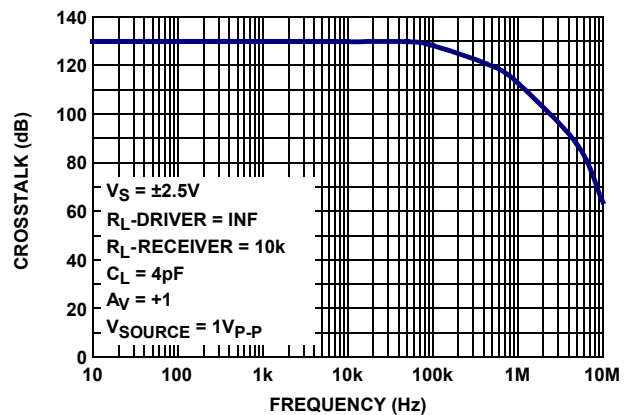
FIGURE 13. CROSSTALK, V_S = \pm 2.5V
