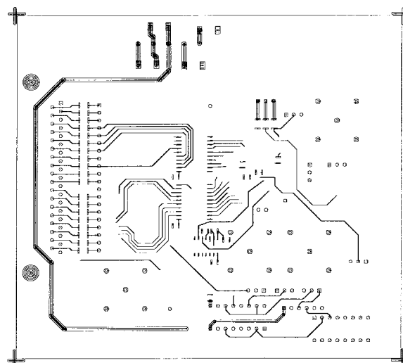
Figure 42. Conductors—Bottom View
