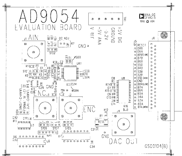
Figure 39. Assembly—Top View
