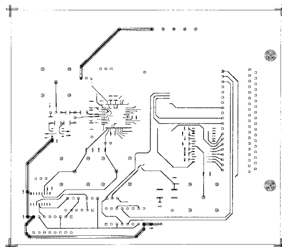
Figure 41. Conductors—Top View
