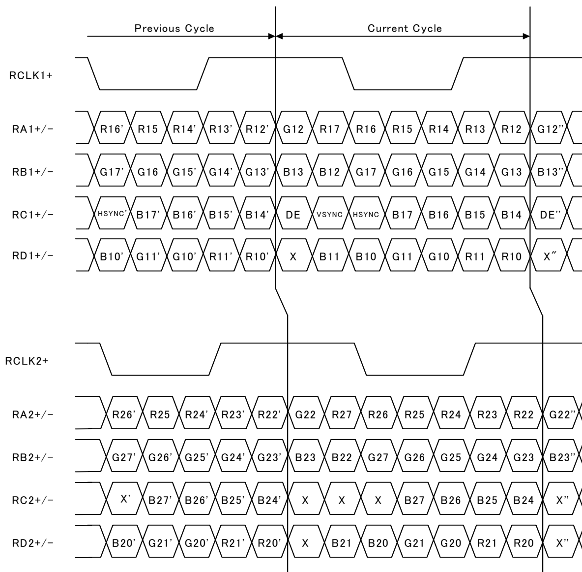
Fig.13 Data Input Timing for Dual Link
