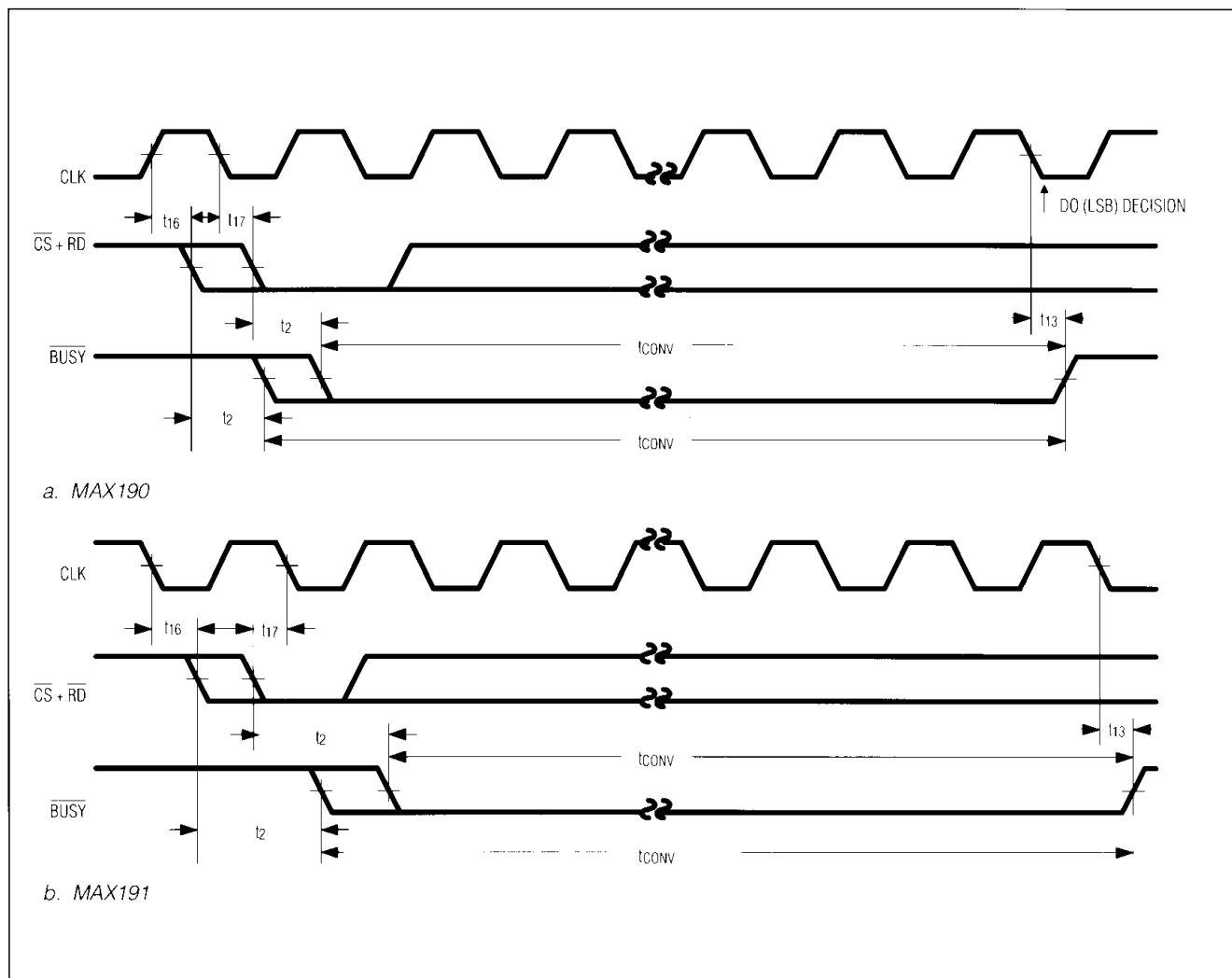
Figure 6. \overline{\text{CS}} , \overline{\text{RD}} , and CLK Synchronous Operation
